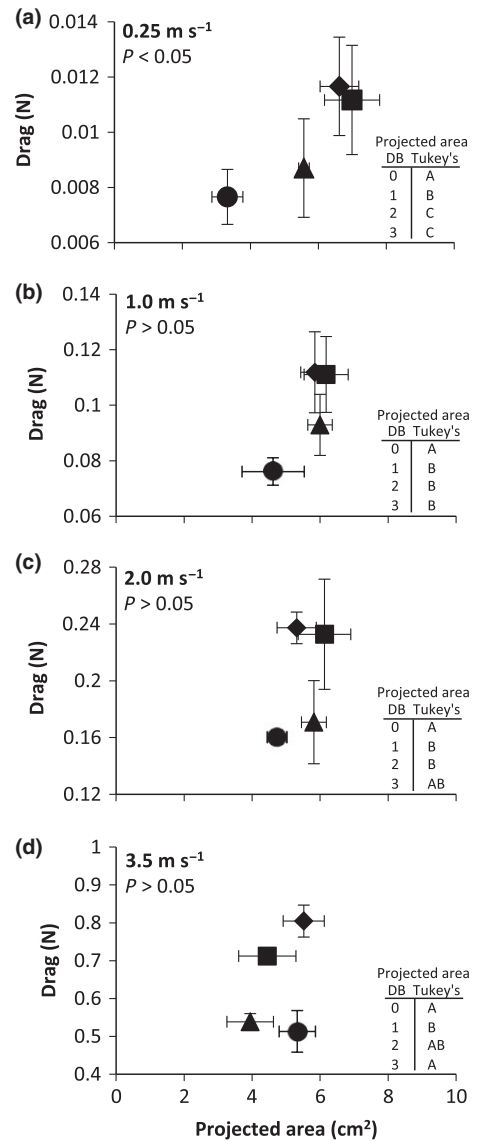
Fig. 3 Effect of projected area on drag experienced by fronds at: (a) 0.25 m s -1 , (b) 1.0 m s -1 , (c) 2.0 m s -1 , and (d) 3.5 m s -1 . Error bars are \pm SD. Shapes represent different branching types: circles, (degree of branching) DB = 0; triangles, DB = 1; squares, DB = 2; diamonds, DB = 3. Different letters within inset tables indicate significant differences (Tukey's honestly significant difference (HSD), P < 0.05 ) in project areas of shapes with different DBs.
